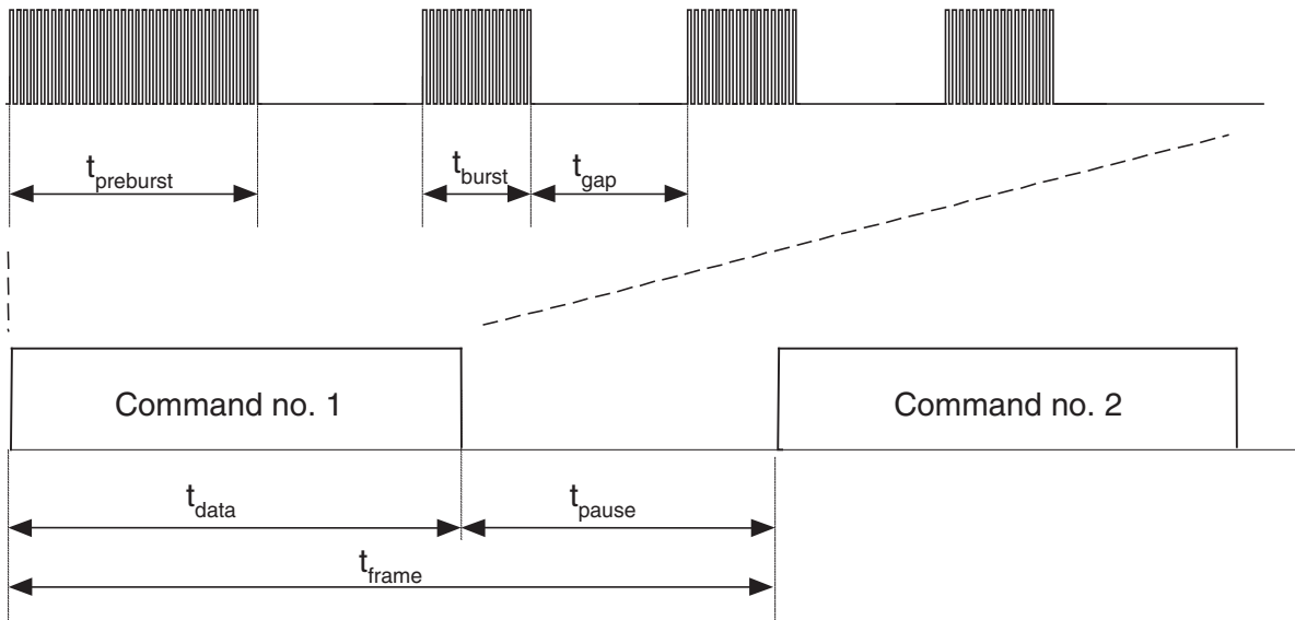
Figure 2-1. Typical IR Signal
