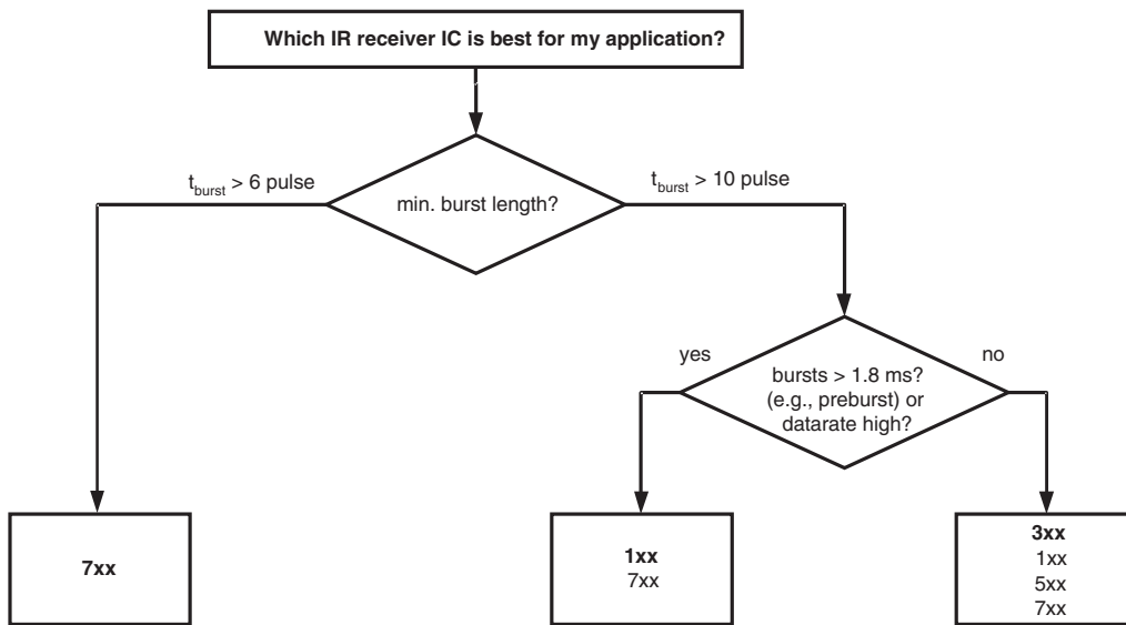
Figure 2-2. IR-code-based Selection Flow
