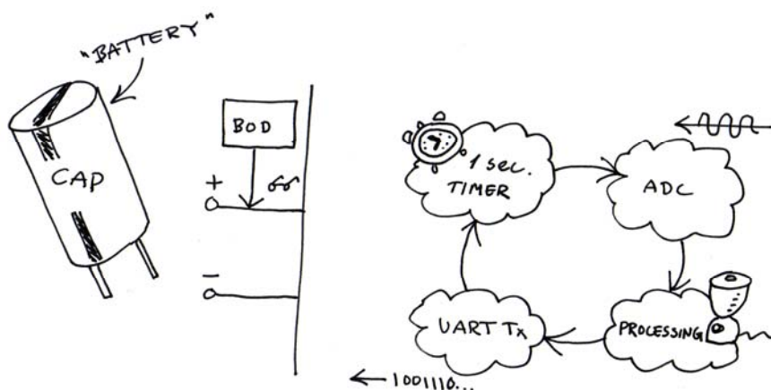
Figure 1-1. Demonstration application
